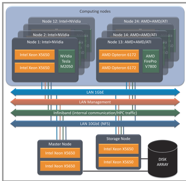
Fig. 2. Hybrid system architecture with Intel+NVIDIA and AMD+ATI/AMD nodes.
