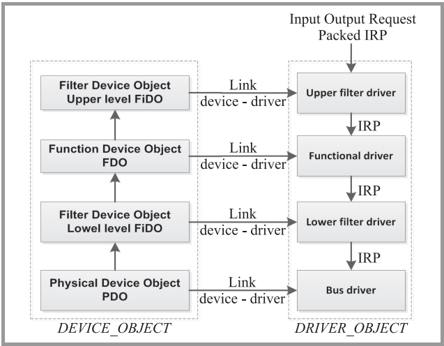
Fig. 4. Windows Driver Model [6].
