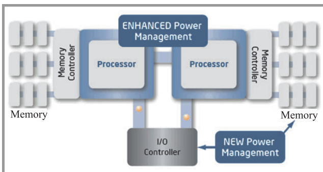
Fig. 3. Block diagram of a system based on the Xeon processor 5600 series.
