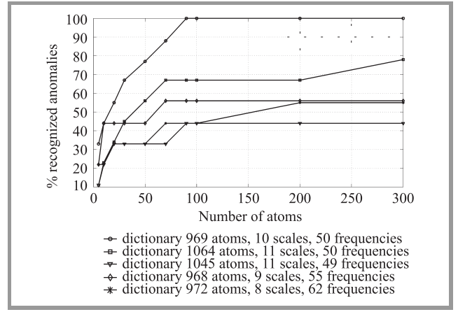
Fig. 2. Percentage of the recognized anomalies as a function of encoded atoms.
