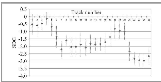
Fig. 5. Subjective fidelity assessment for the signal with the embedded watermark. The results are provided for the confidence interval of 95% and were determined with use of the ITU-R BS 1116-1 test. Details about sound tracks used in this test can be found in Table 1.
