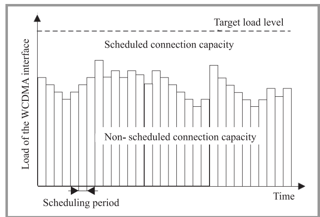
Fig. 4. Illustration of cell-specific packet scheduler.
