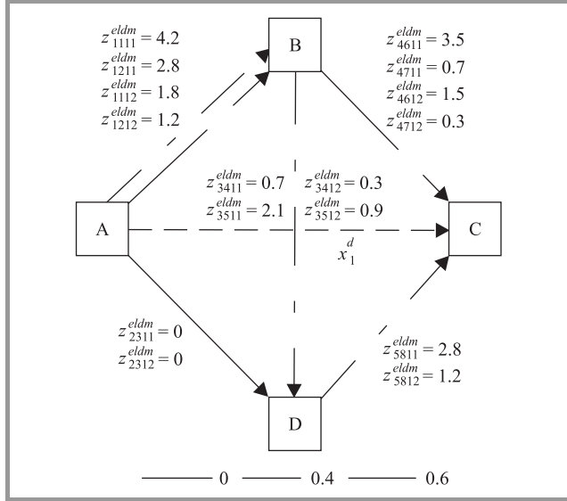
Fig. 7. Exemplary solution of the second stage of disaggregation model. We can see z_{e_l d_m} variables ( z_{xxxx}^{eldm} ) which are realization of m th buy offer (which belongs to the demand d ) by the l th sell offer (which belongs to the link e ).
