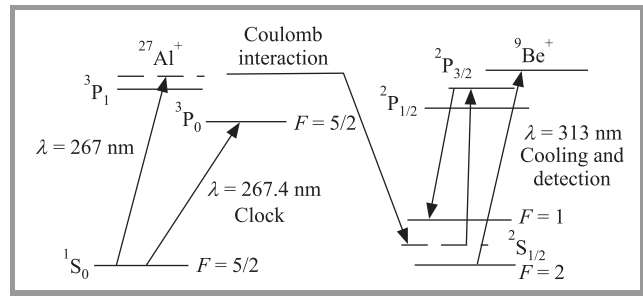
Fig. 4. Transfer of the ^{27}\text{Al}^+ clock state to detectable states in ^9\text{Be}^+ [16].
