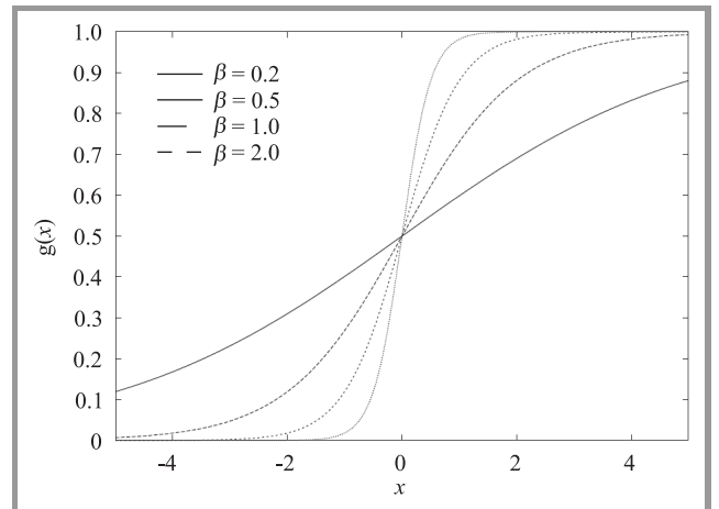
Fig. 5. Activation function.
