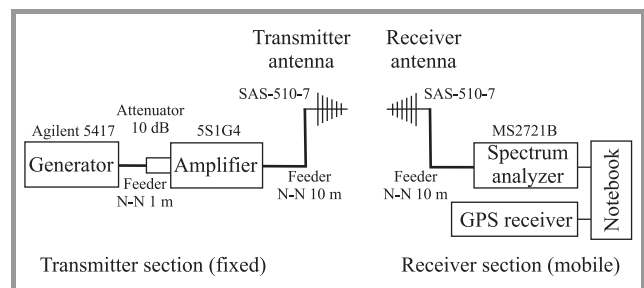
Fig. 1. Block diagram of primary measuring equipment set.
