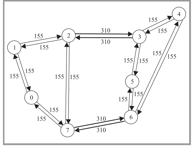
Fig. 4. Test network \mathcal{M} [45], with the indication of the bandwidth of each arc C'_k [Mbit/s].
