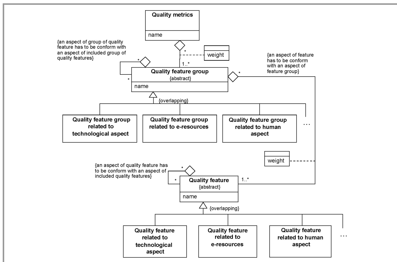
Fig. 1. The idea of quality metrics.
