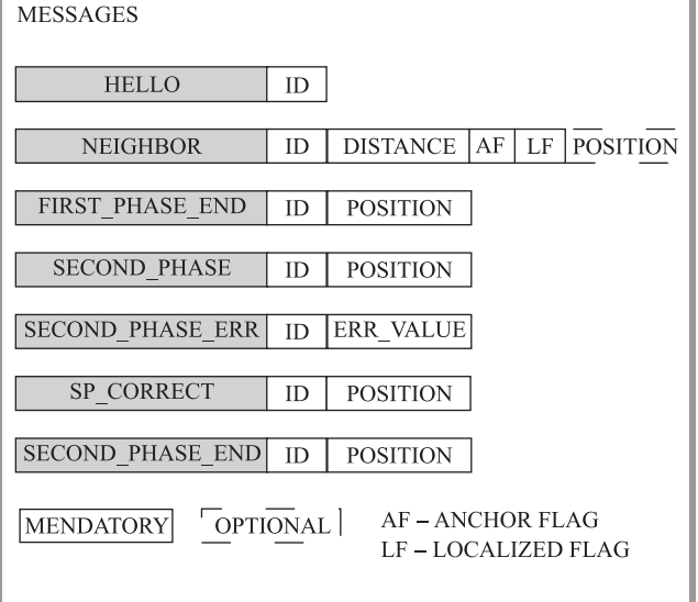
Fig. 2. The scheme of exchanged messages.
