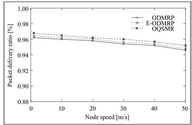
Fig. 15. Packet delivery ratio vs. node speed (1 group, 1 source, 20 multicast receivers).
