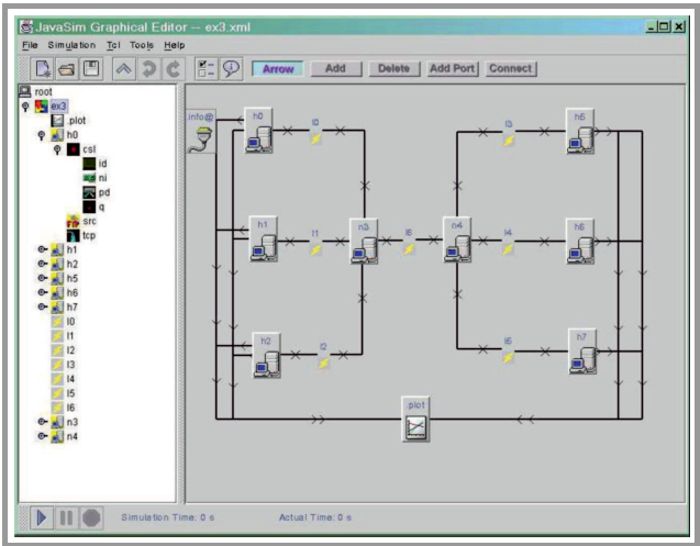
Fig. 8. J-Sim gEditor application example.
