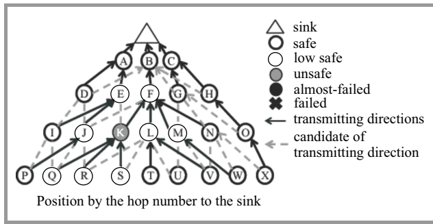
Fig. 3. Destination node selection with unsafe nodes.
