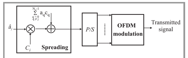
Fig. 3. MC-CDMA transmitter.
