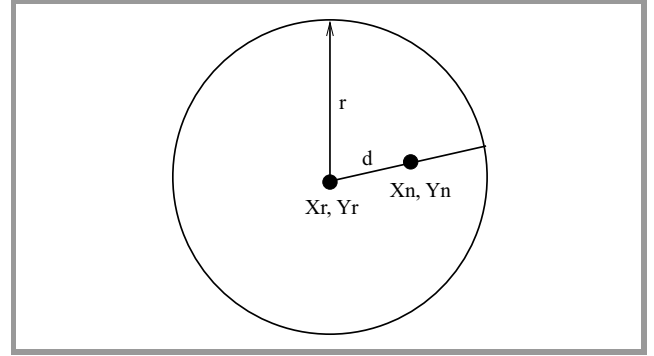
Fig. 1. Node movement.
