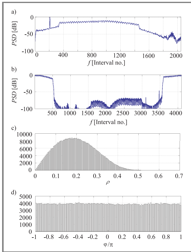
Fig. 1. A typical HF OFDM signal: (a) spectrum; (b) spectrum after preprocessing; (c) histogram of magnitude \rho , time domain; (d) histogram of phase \varphi/\pi , time domain.
