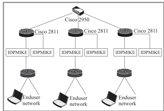
Fig. 3. The realized test-bed.
