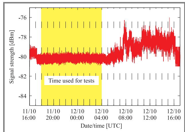
Fig. 2. Example for received signal strength from node B on node C during 24 hours. Signal strengths are averaged over 10 s; time is UTC (coordinated universal time).
