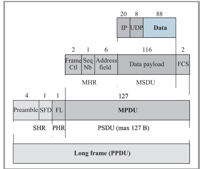
Fig. 7. Structure of an IEEE 802.15.4 data frame. Explanations: MSDU – MAC service data unit, PSDU – PHY service data unit, PPDU – PHY protocol data unit.
