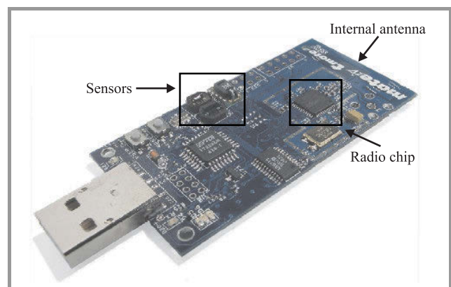
Fig. 3. Tmote TM Sky platform from Moteiv.
