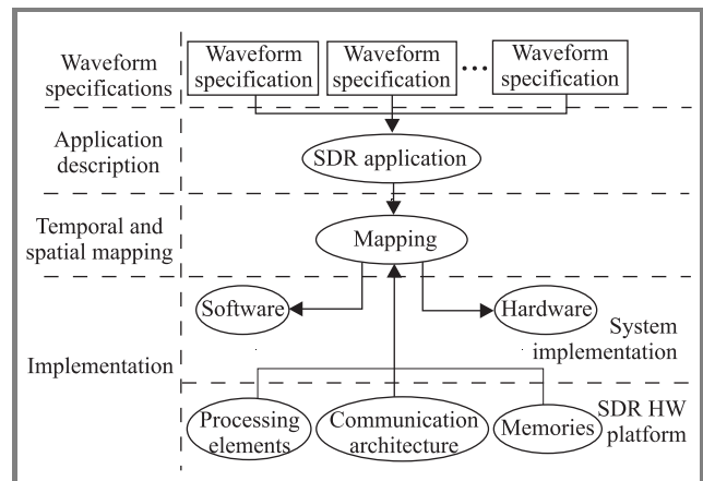
Fig. 2. Design flow from application description to implementation.
