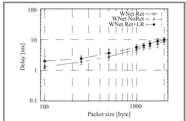
Fig. 14. Simulated delay versus packet size for three WNet variants at 200 kbit/s.
