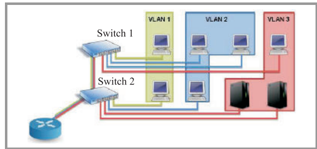
Fig. 2. An example of VLAN virtualization at layer 2.
