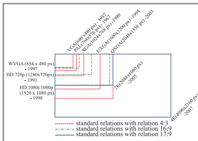
Fig. 1. Standards for image resolution.
