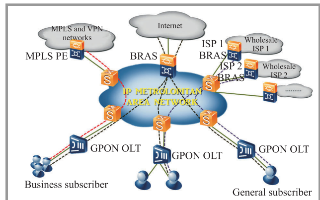
Fig. 6. Wholesale subscriber access via VLAN stacking.
