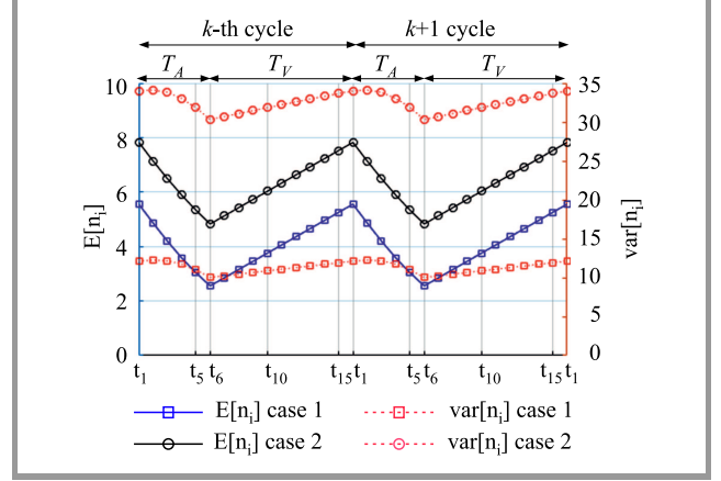
Fig. 8. Mean E[n_i] and variance \text{var}[n_i] of packets in the system at times t_i ( i = 1, 2, \dots, N ).
