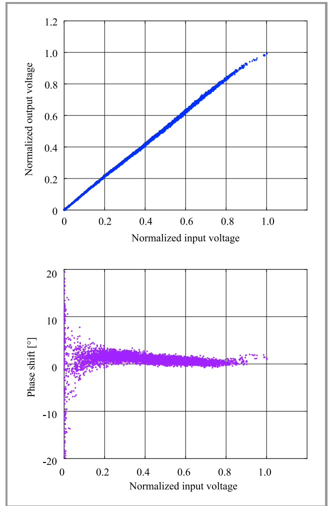
Fig. 12. Linearized AM/AM and AM/PM characteristics using FWMP model.
