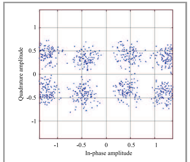
Fig. 3. Constellation diagram OFDM NOMA signals.
