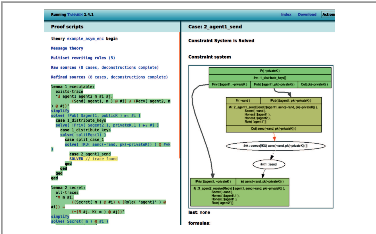
Fig. 1. Tamarin tool interactive mode.
