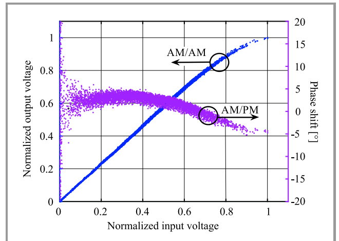
Fig. 6. Instantaneous AM/AM and AM/PM characteristics for an 64-QAM input signal with 7.5 dB PAPR.
