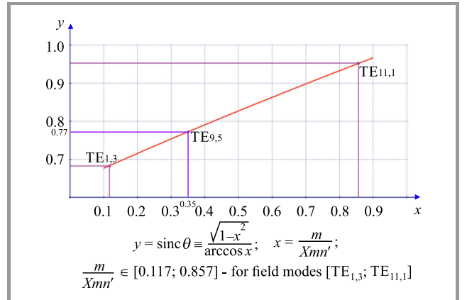
Fig. 14. Visualization of the value of the y = \text{sinc } \theta function for the selected field mode, represented by x = \frac{m}{\chi_{mn'}} .
