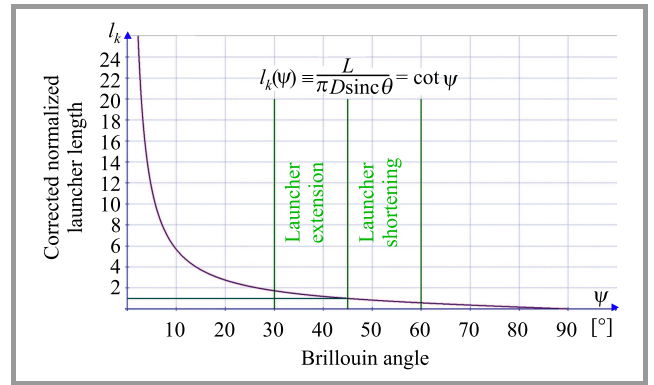
Fig. 8. Relationship between normalized launcher length l_k and the Brillouin angle \psi .
