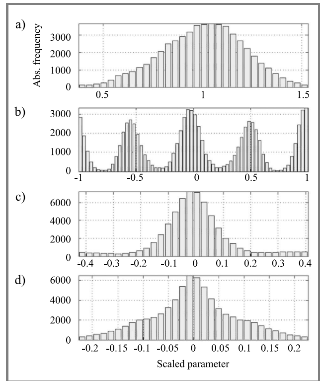
Fig. 4. Parameter histograms for PSK4: (a) amplitude a ; (b) difference phase D\phi ; (c) instantaneous frequency f ; (d) differential instantaneous frequency df .
