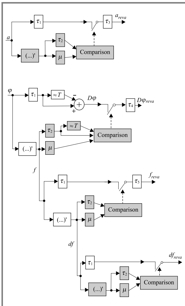
Fig. 3. Feature extraction, non-synchronized.
