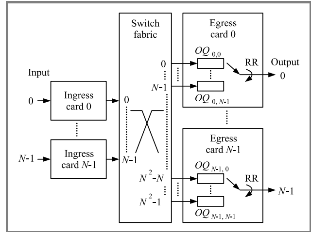
Fig. 1. The switch architecture with multiple output queueing.
