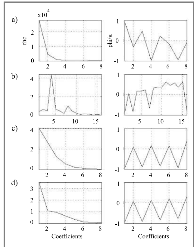
Fig. 5. Picture functions for PSK4: (a) amplitude a ; (b) difference phase D\phi ; (c) instantaneous frequency f ; (d) differential instantaneous frequency df .
