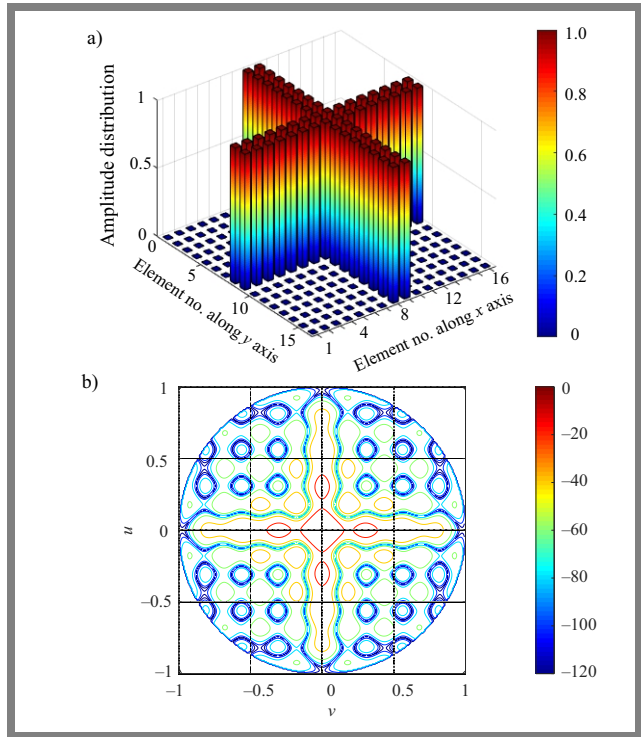
Fig. 4. Proposed plus-shaped receive array and its corresponding contour pattern.
