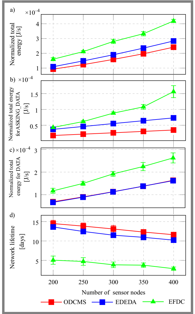
Fig. 8. Comparison of simulation results for ODCMS, EDEDA, and EFDC protocols across multiple scenarios (with standard deviation error bars).
