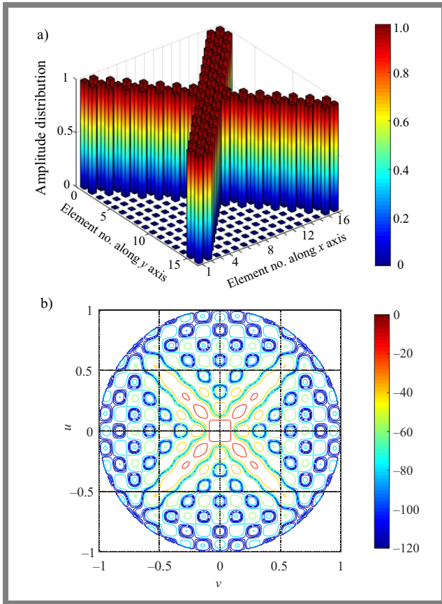
Fig. 3. Proposed X-shaped receive antenna array structure and its corresponding contour pattern.
