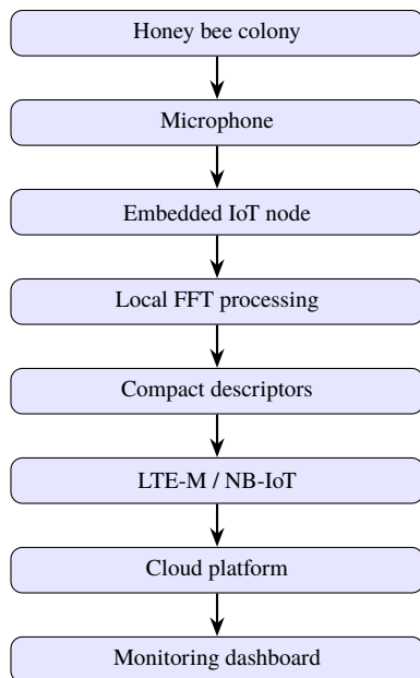
Fig. 2. Architecture of the proposed embedded acoustic telemetry framework.
