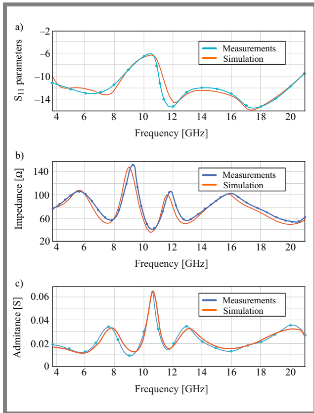
Fig. 8. S_{11} for the proposed antenna a), input impedance b), and admittance c).
