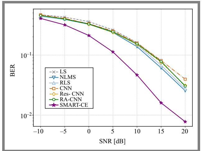
Fig. 5. BER performance over the spatially correlated MIMO channel.
