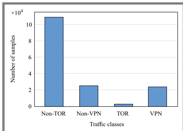
Fig. 2. Distribution of traffic categories in the Darknet 2020 dataset.
