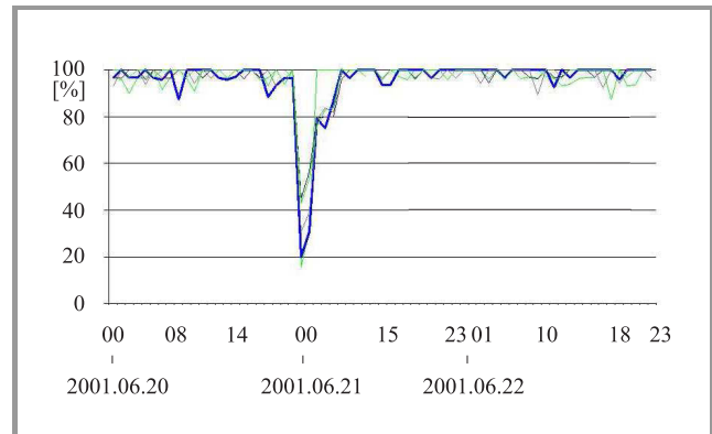
Fig. 4. Successful call ratio – relation from network area to the outside area.
