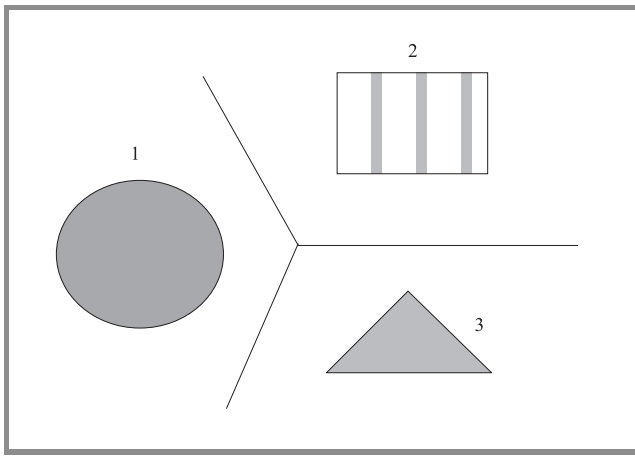
Fig. 1. Segmentation.
