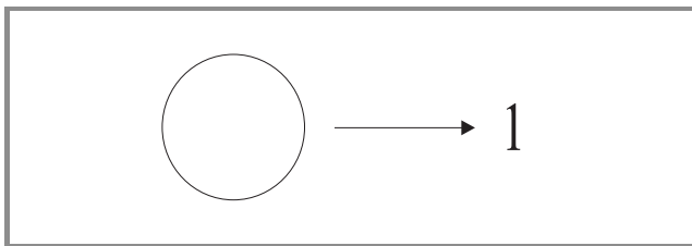
Fig. 2. Classification.
