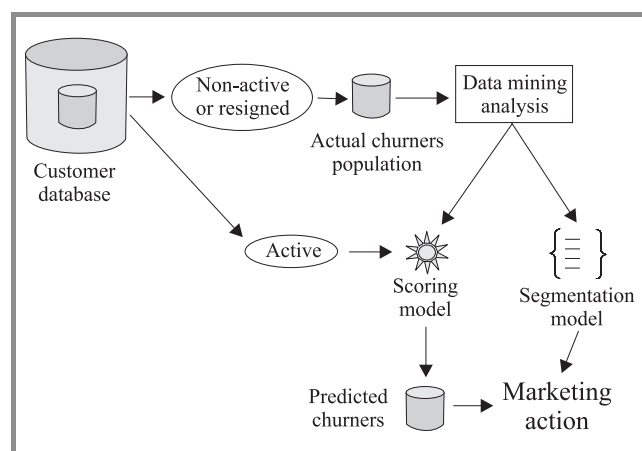
Fig. 6. Segmentation model.
