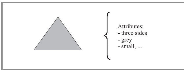
Fig. 3. Profiling.
