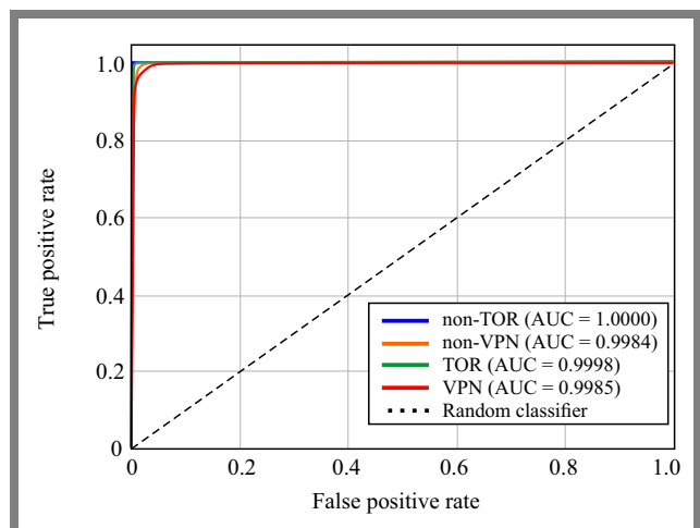
Fig. 4. ROC curves and corresponding AUC values for four types of traffic.
