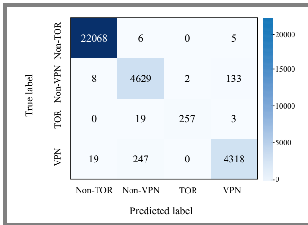
Fig. 3. Confusion matrix of the XGBoost model.
