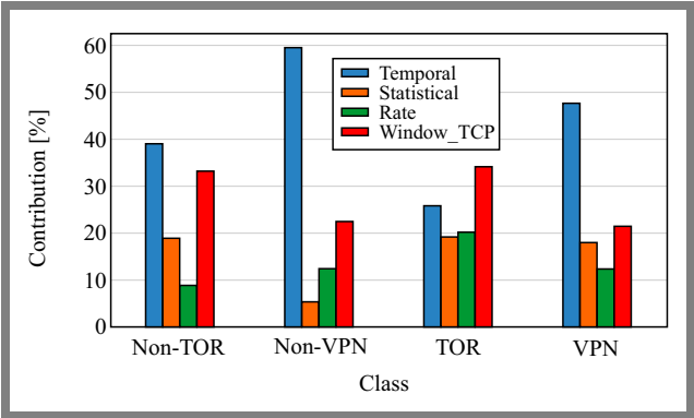
Fig. 6. Category-SHAP contribution analysis across traffic classes.
