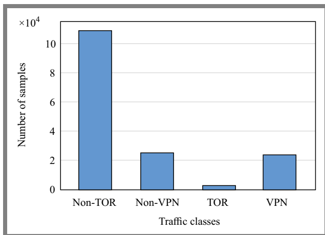
Fig. 2. Distribution of traffic categories in the Darknet 2020 dataset.
