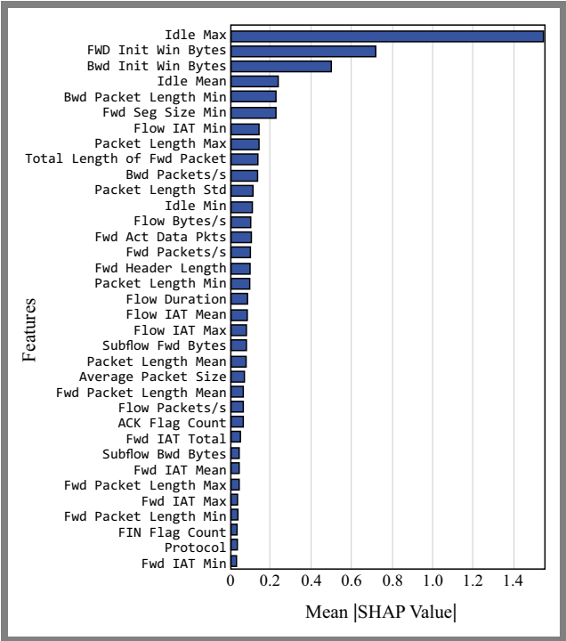
Fig. 5. 35 selected features representing 95% cumulative SHAP importance.
